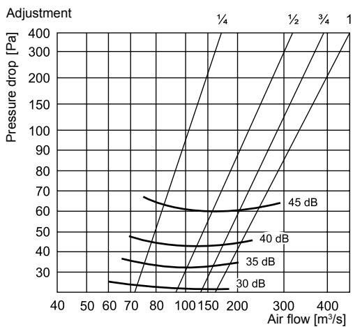
P-DVS 160
