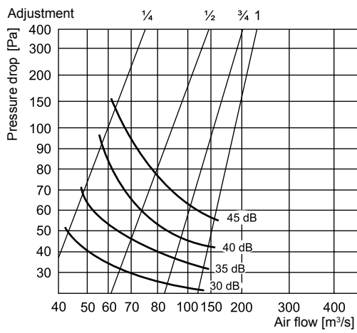
P-DVS 100
